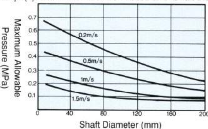
Graph(5): Maximum Allowable Pressure vs. Shaft Diameter
