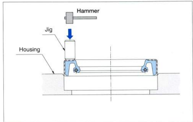
Figure 17: Seal Installation
