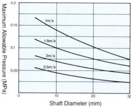
Graph(4): Maximum Allowable Pressure vs. Shaft Diameter
