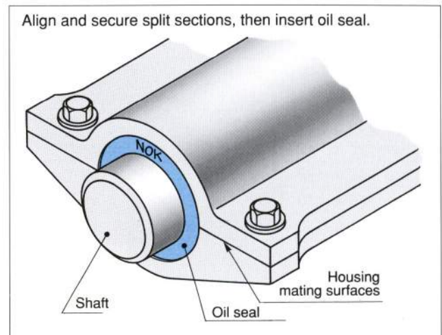
Figure 2: Split-Type Housing
