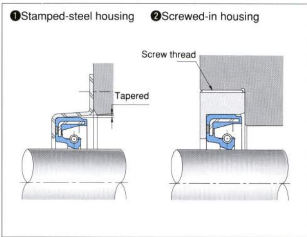
Figure 3: Improper Housing Bore Designs
