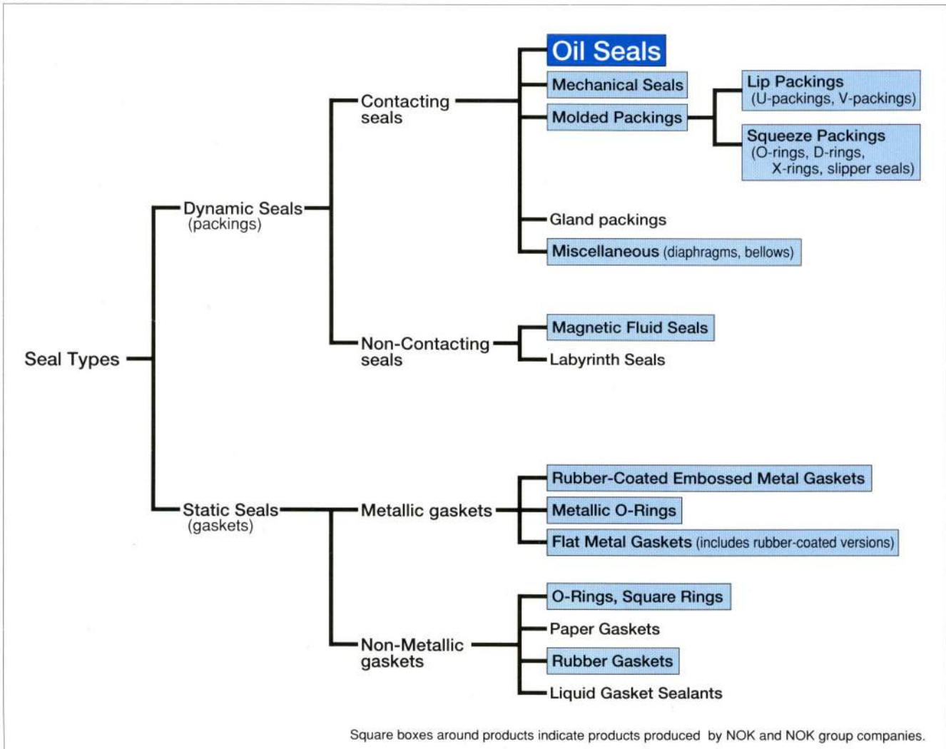
Figure 1: Seal Classifications
