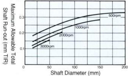
Graph(7): Maximum Allowable Total Shaft Run-out vs. Shaft Diameter
